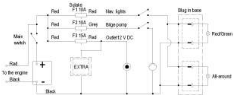
Figure 6. Terhi 475 wiring diagram
