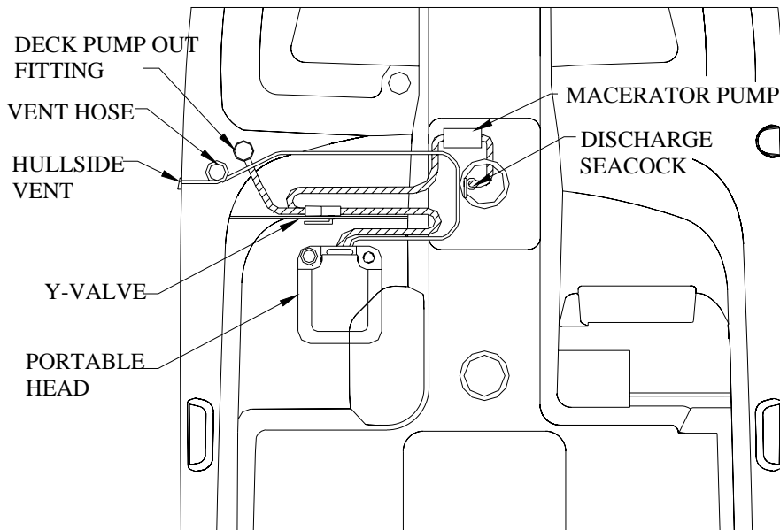
PORTABLE HEAD W/ IN-LINE MACERATOR
