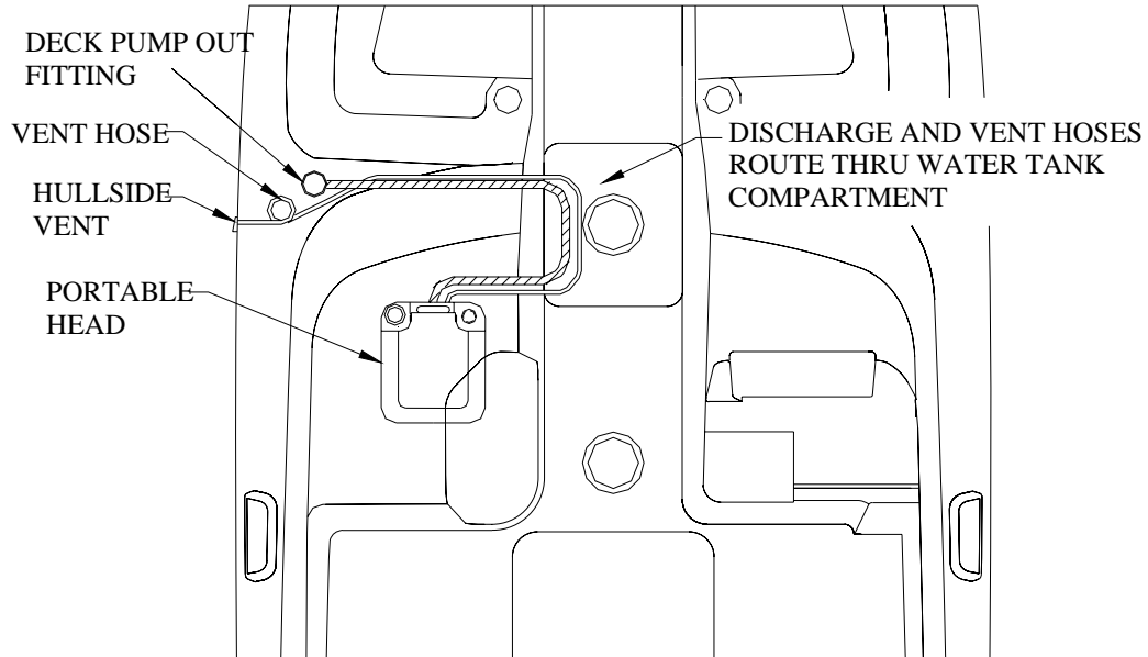
PORTABLE HEAD W/ DECK PUMP OUT
