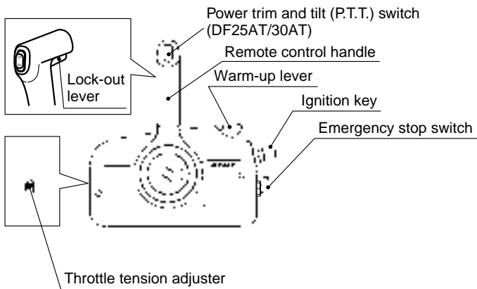
REMOTE CONTROL BOX (DF25AR/25AT/30AR/30AT)
