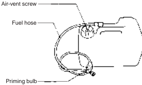
FUEL TANK
