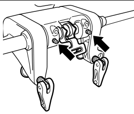
Swivel bracket
