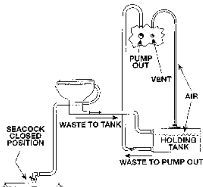
FIGURE 3.10 TYPICAL HEAD DISCHARGE SYSTEM
