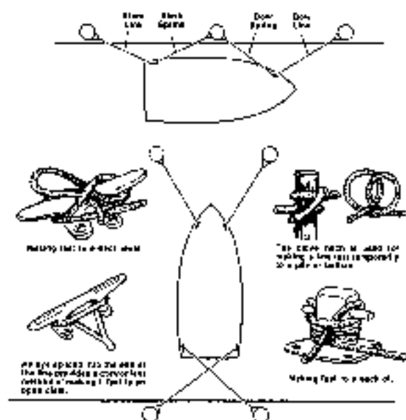
FIGURE 5.9 MOORING LINES
