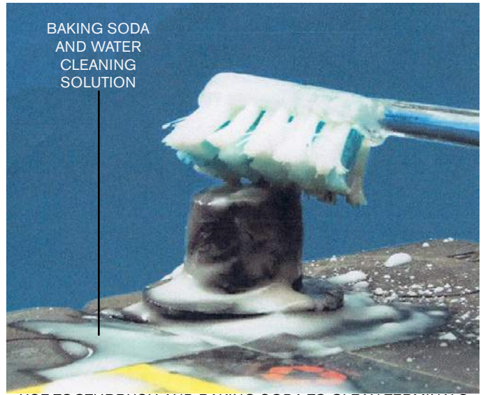
USE TOOTHBRUSH AND BAKING SODA TO CLEAN TERMINALS
