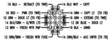
TO LEFT (PORT) SWP (W/ SOC)
