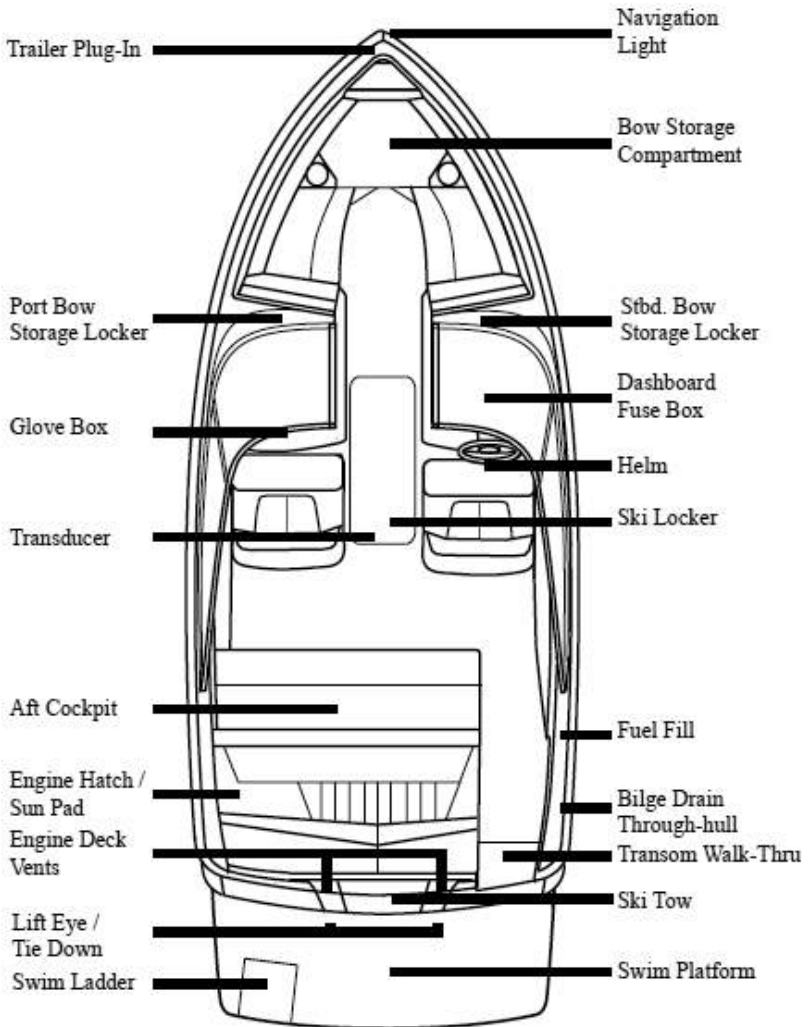
Plan View
