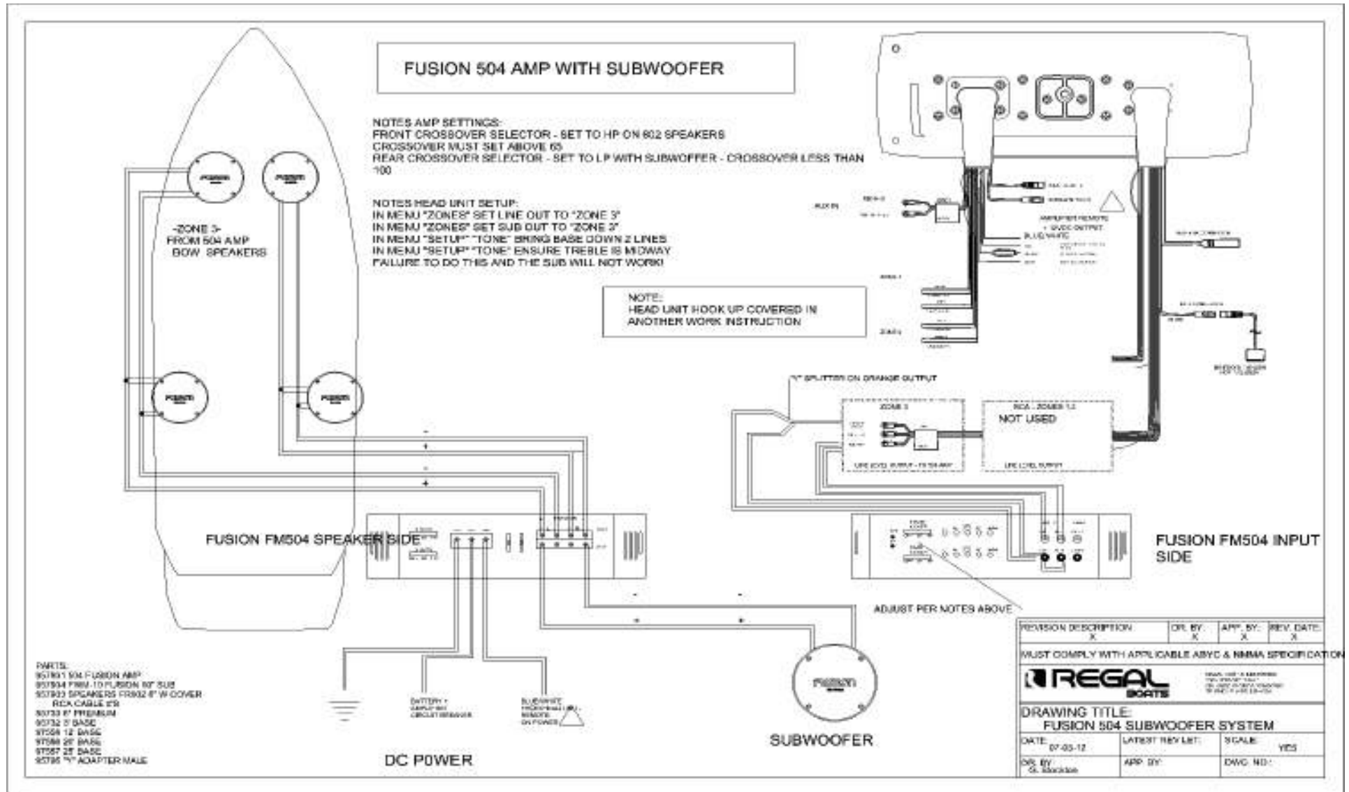
Fusion Stereo Optional Performance Package Connection
