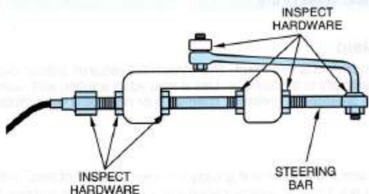
TYPICAL ENGINE STEERING LINK
