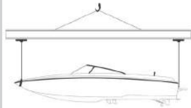
CORRECT HOISTING
