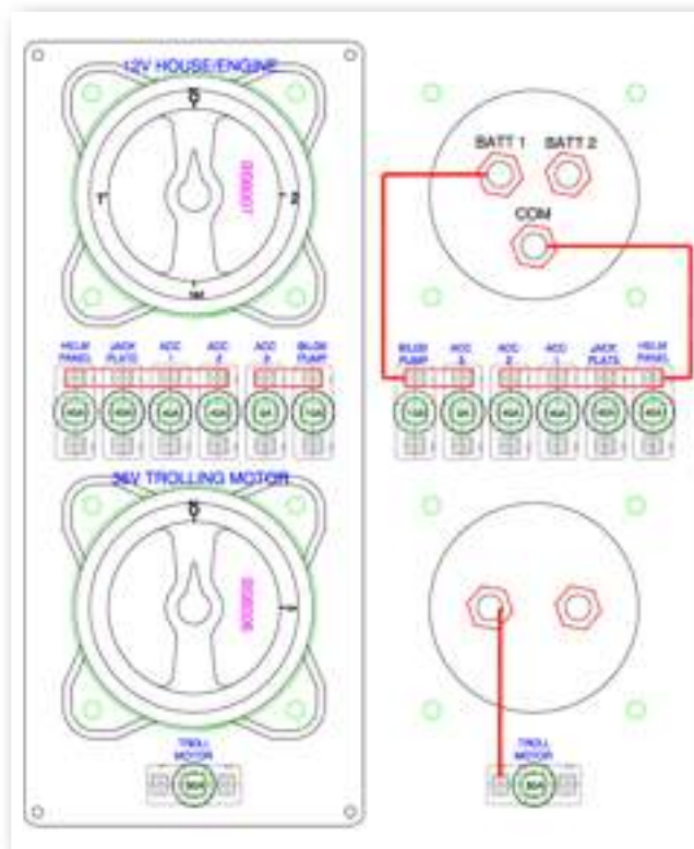
Battery Switch Diagram
