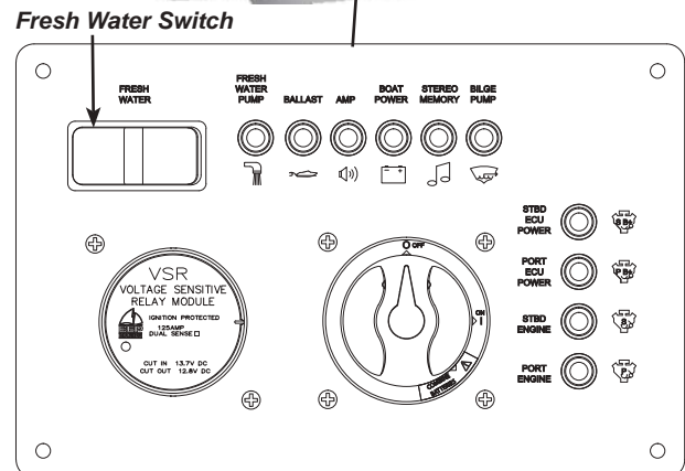
Figure B44: Fresh Water Switch on Battery Switch Panel
