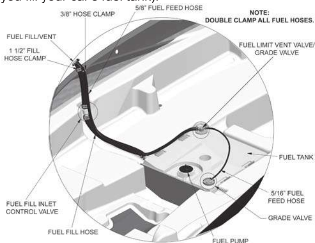
Figure B32: Pressurized Fuel System
