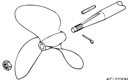
Figure 3-13. Propeller
