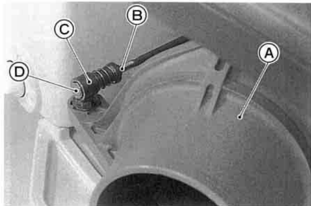
A. Steering Nozzle B. Locknut C. Sleeve D. Ball Joint
