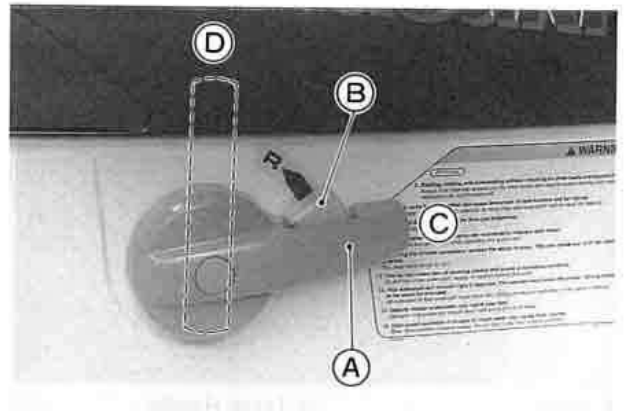
A. Shift Lever B. Trigger C. F(Forward) position D. R(Reverse) position
