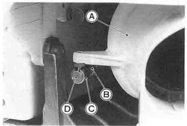
A. Steering Nozzle C. Sleeve B. Locknut D. Ball Joint
