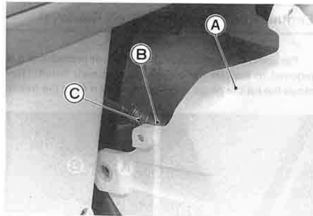
A. Reverse Bucket C. Ball Joint B. Sleeve
