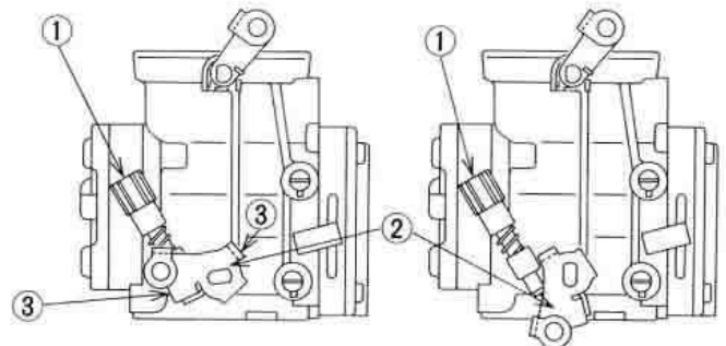
THROTTLE CLOSED (RELEASED)
