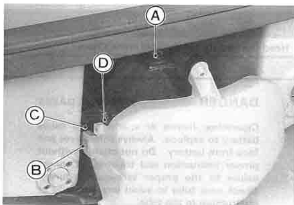
A. Steering Nozzle Pivots C. Steering Link Ball Joint B. Reverse Bucket Pivots D. Shift Link Ball Joint
