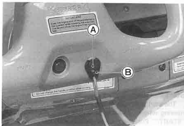
A. Engine Shut-off Switch B. Lanyard Key
