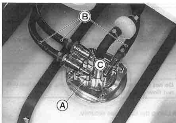
A. Fuel Outlet Assembly C. Screws B. Fuel Hoses
