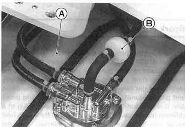
A. Fuel Tank B. Check Valve
