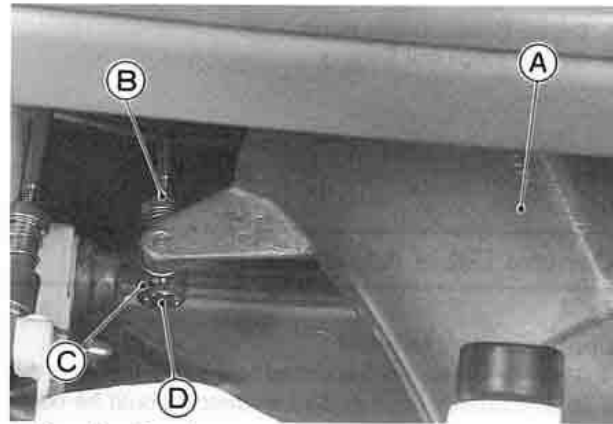
A. Steering Nozzle C. Sleeve B. Locknut D. Ball Joint
