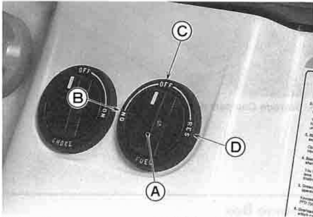
A. Fuel Knob B. ON position C. OFF position D. RES position
