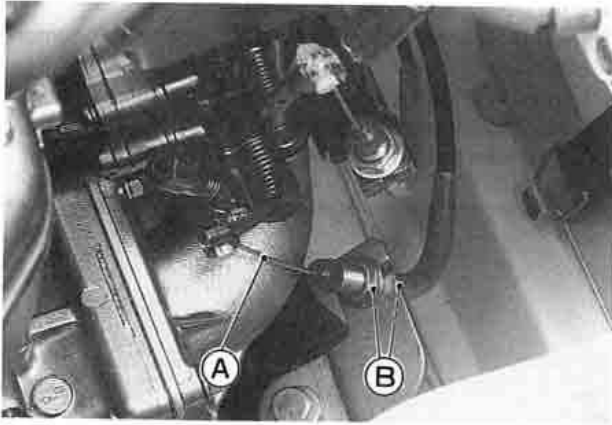
A. Throttle Cable B. Locknuts
