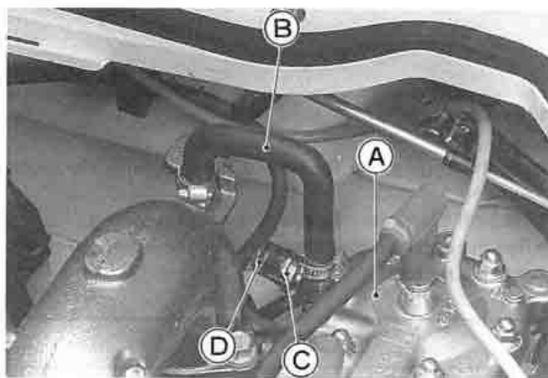
A. Cylinder Head B. Cooling Hose C. Clamp D. Cap
