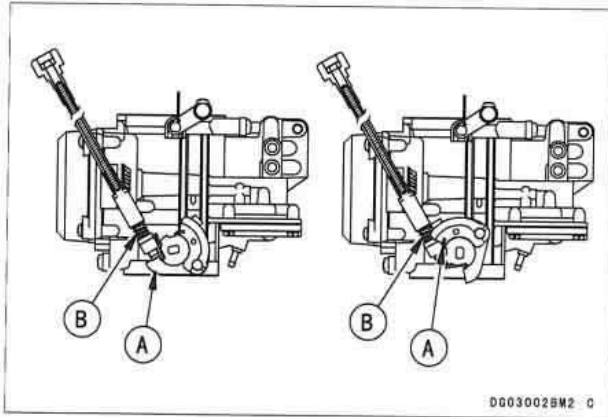
THROTTLE CLOSED (RELEASED)
