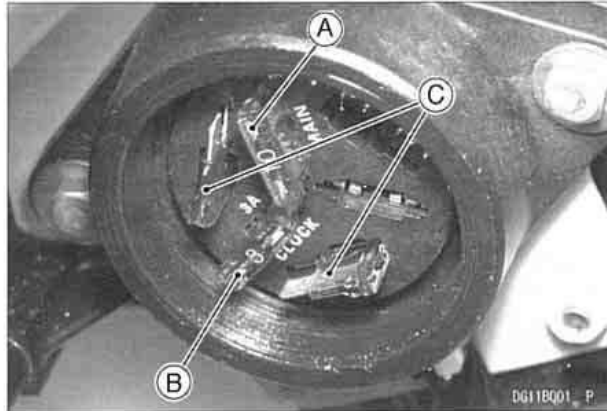
A. Main Fuse B. Clock Fuse
