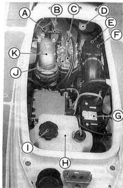
A. Drain Valve Knob B. Cooling Hose C. Spark Plugs D. Sediment Bowl E. Flame Arrester F. Carburetor G. Battery H. Oil Tank I. Oil Filler Cap J. Cylinder Head K. Exhaust Pipe
