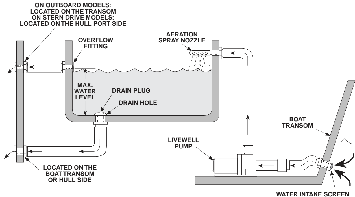
FIGURE 2.9 MANUAL LIVEWELL
