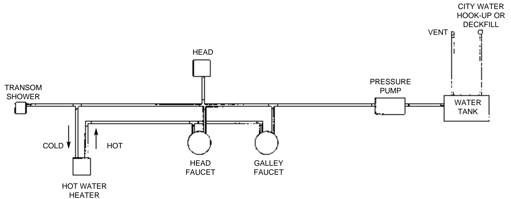
FIGURE 2.6 – TYPICAL PLUMBING DIAGRAM
