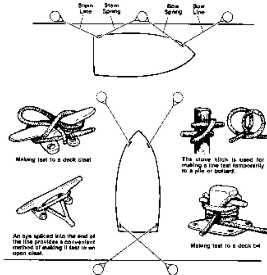
FIGURE 3.1 MOORING LINES
