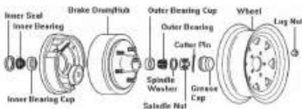
Figure P13: Axle Components
