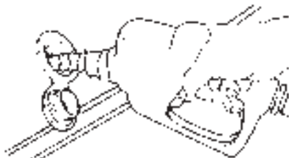
Grounding the fuel hose - Proper
