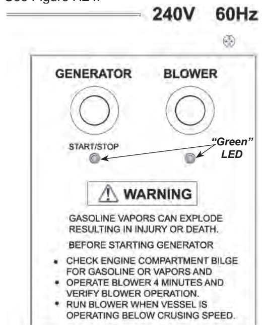
Figure H24: Remote Generator & Blower Switches
