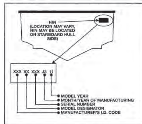
Figure A7: HIN
