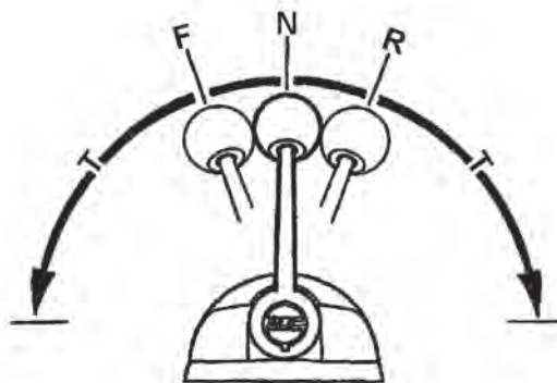
Figure F3: Electronic Control Lever Positions
