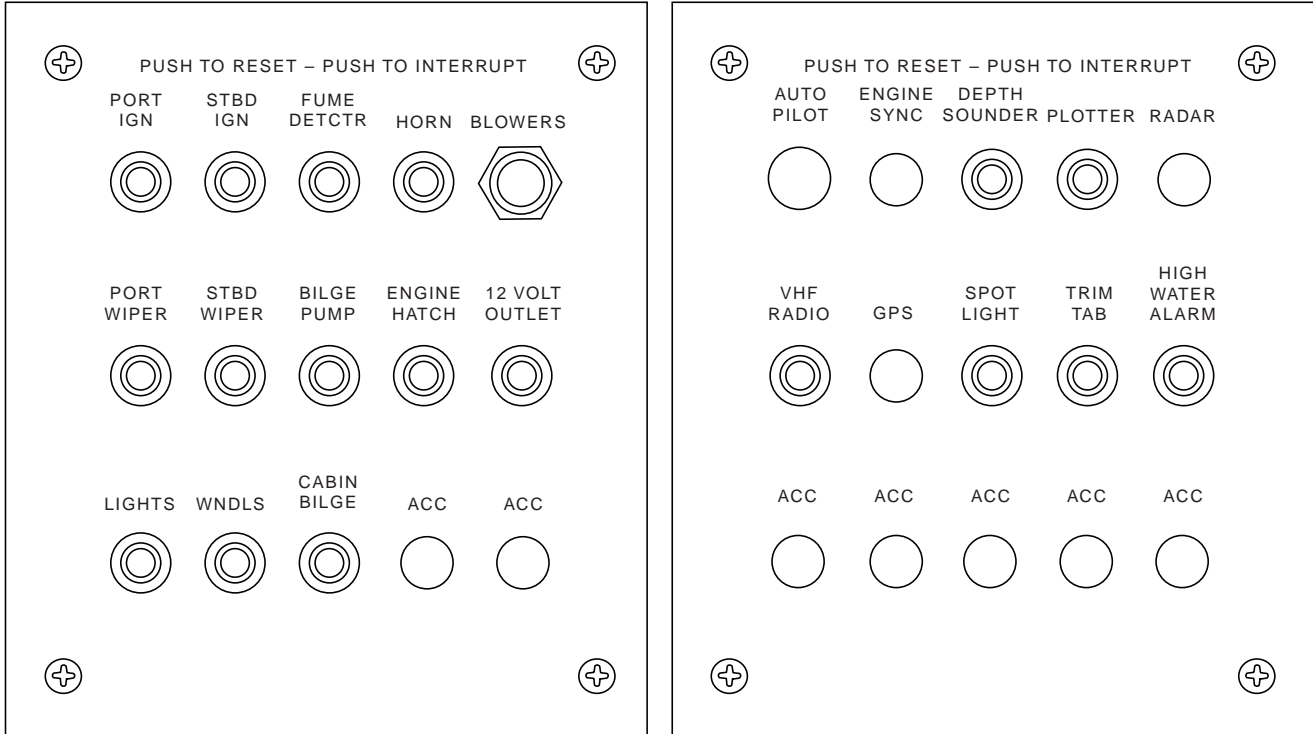
Typical Circuit Breaker Panel Figure 4-19
