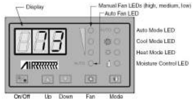
AC Control Pod Figure 5-10
