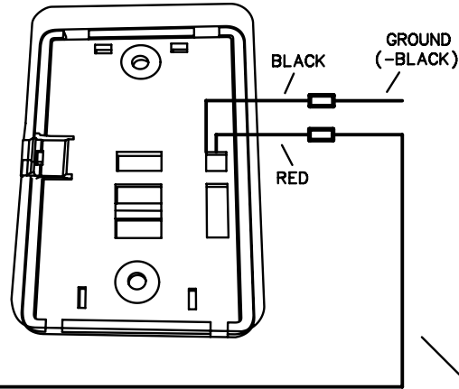
CO DETECTOR (REAR VIEW)
