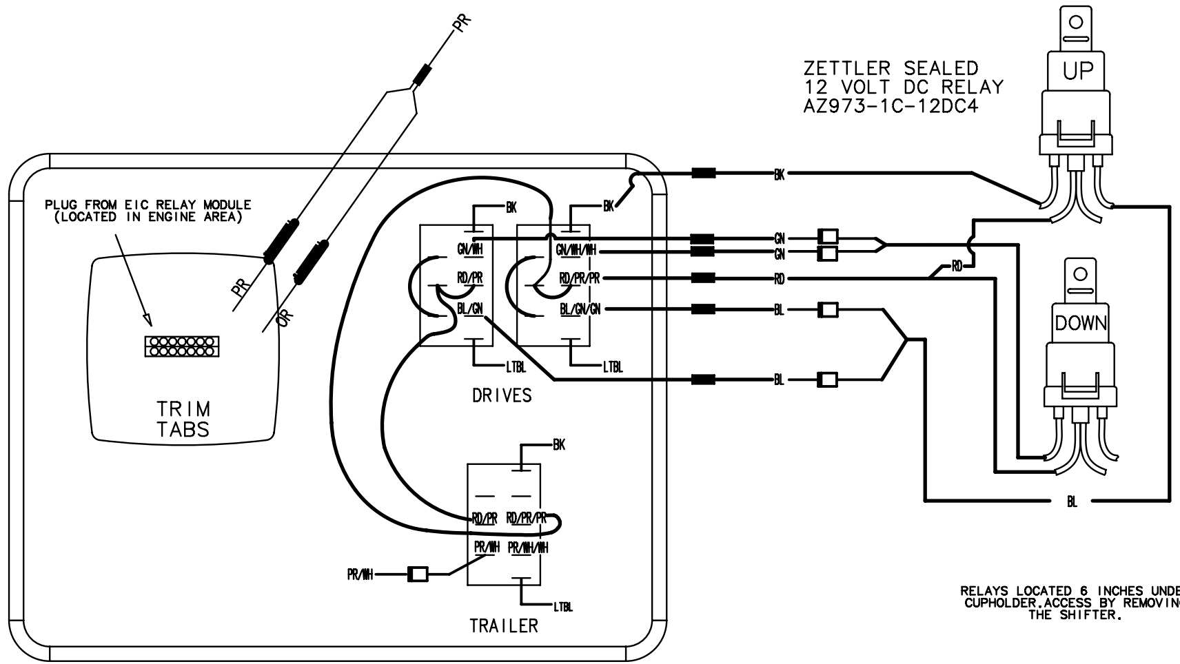
TRIM PANEL (REAR VIEW)
