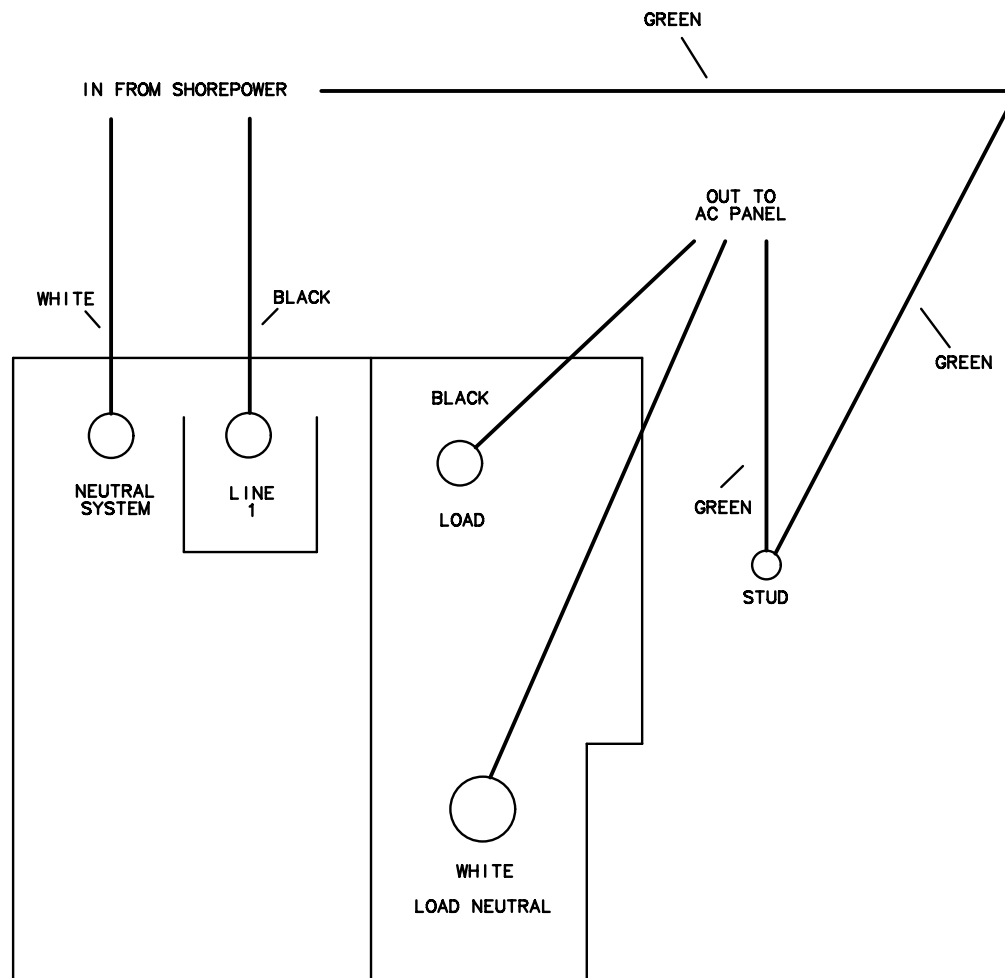
SHOREPOWER ELCI BREAKER (REAR VIEW)
