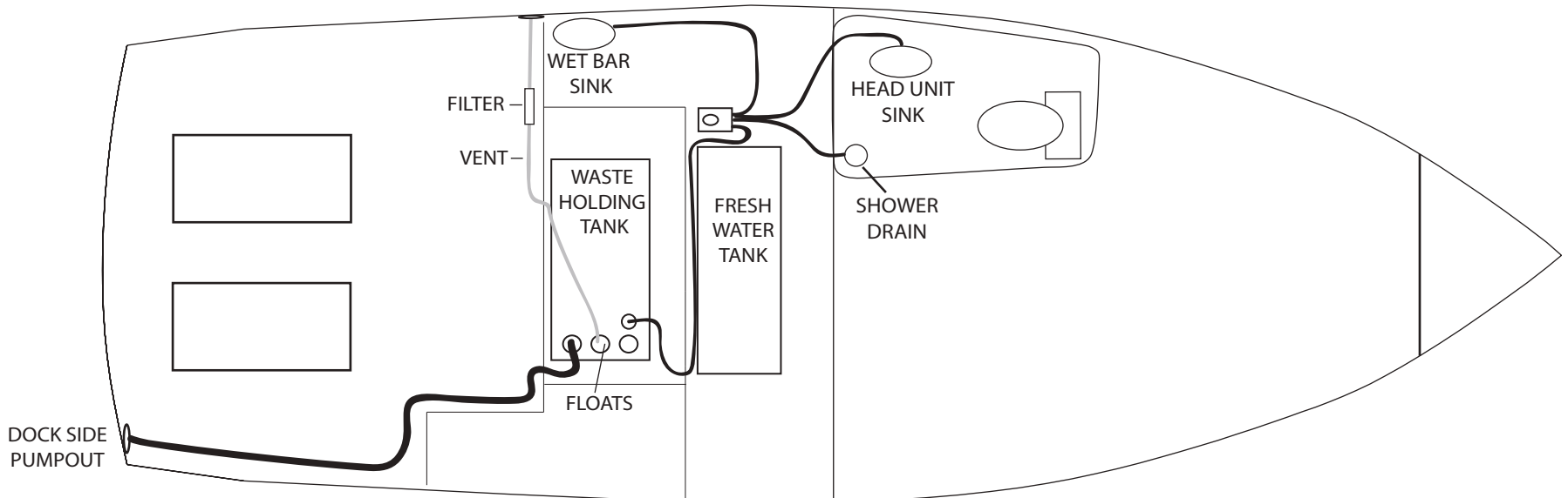
GRAY WATER OPTION
