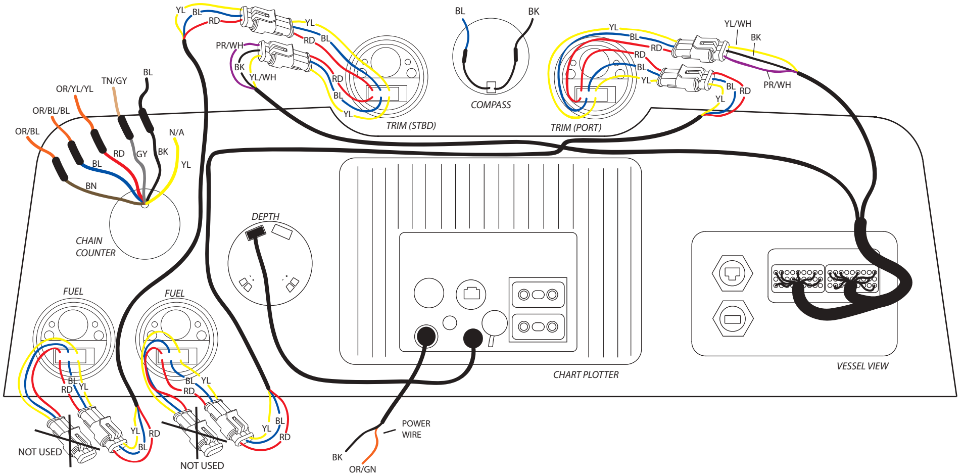
(REAR VIEW)
