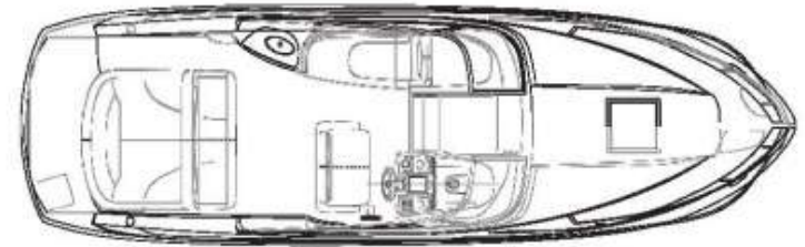
SIGNATURE 270 OPTIONAL DECK PLAN
