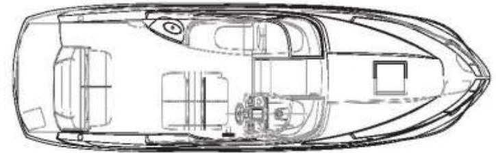
SIGNATURE 270 STANDARD DECK PLAN
