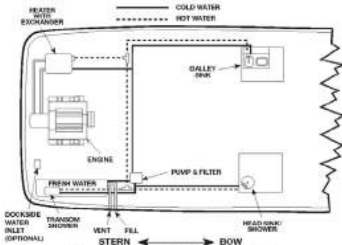
Figure 3.3 Potable Water System
